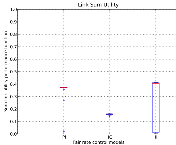
Figure 8.12: Sum utility
